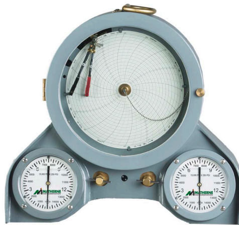
12" Circular Chart Recorder, Portable, with 5" Pressure Gauges
